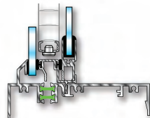
S1500 Strut Fixed Window
