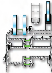
S6800 Strut In-swing Triple-glazed Casement/Projected Window Hinged-panel option with 3/4" blinds Fixed version available
