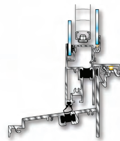
3400 Tilt Double-Hung Window
