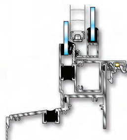
2500 Side-load Double-Hung Window Hinged-panel option
