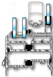
6800 In-swing Triple-glazed Casement/Projected Window Hinged-panel option with 1" blinds Fixed version available
