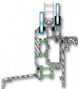
S2500 Strut Side-load Double-Hung Window
