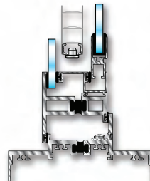
6900 Out-swing Casement/Projected Window Lift & tuck panel option with 3/4" blinds Fixed version available
