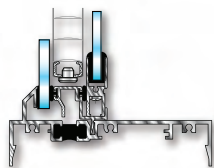
1500 Fixed Window
