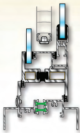
6000 Out-swing Casement/Projected Window Fixed version available
