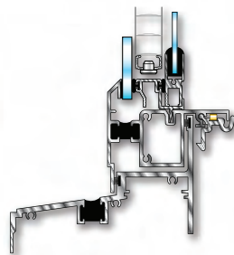
2500 Side-load Double-Hung Window
