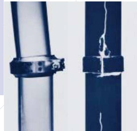
Left: KIMAX Couplings provide leak-free seals even when deflected up to 4°. Right: Plastic systems do not provide joint deflection capability.
