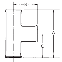
STRAIGHT T 6523
