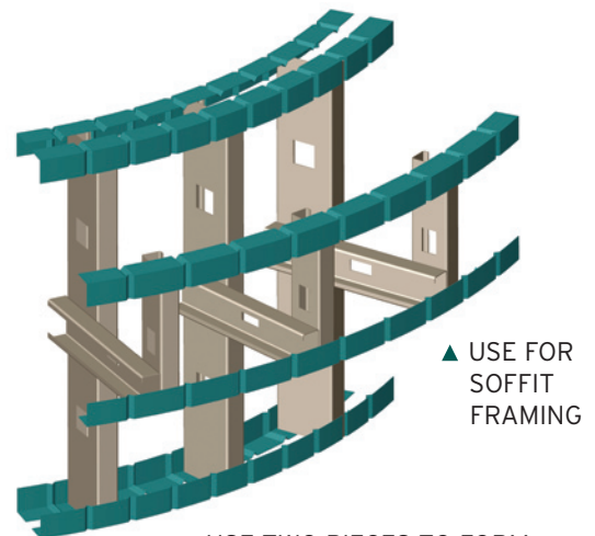
▲ USE TWO PIECES TO FORM CURVED TRACKS AND ARCHES
