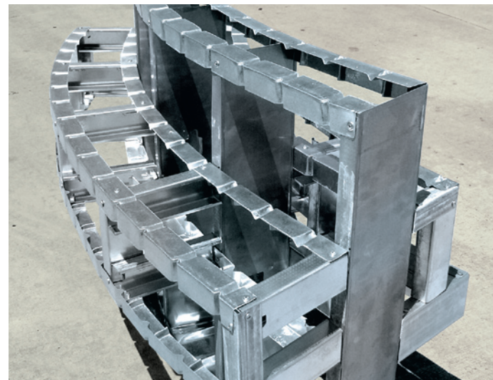
TWO LENGTHS OF READY-ANGLE FORM A DOOR OR WINDOW ARCH
