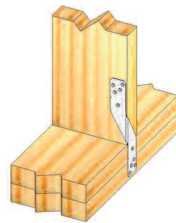
Typical RT8A stud to double plate installation
