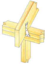
Typical RT3 truss/rafter to plate installation
