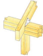
Typical RT6 truss/rafter to double plate installation
