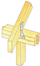
Typical RT7 truss/rafter to double plate installation
