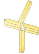
Typical RT5 truss/rafter to double plate installation
