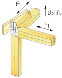
Typical HHCP2 truss/rafter to double plate corner installation
