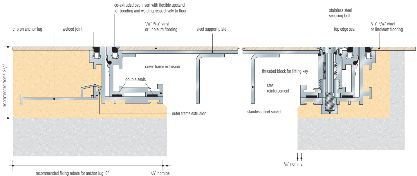
Cross section showing anchor lug and locking/lifting detail (scale 1:2)
