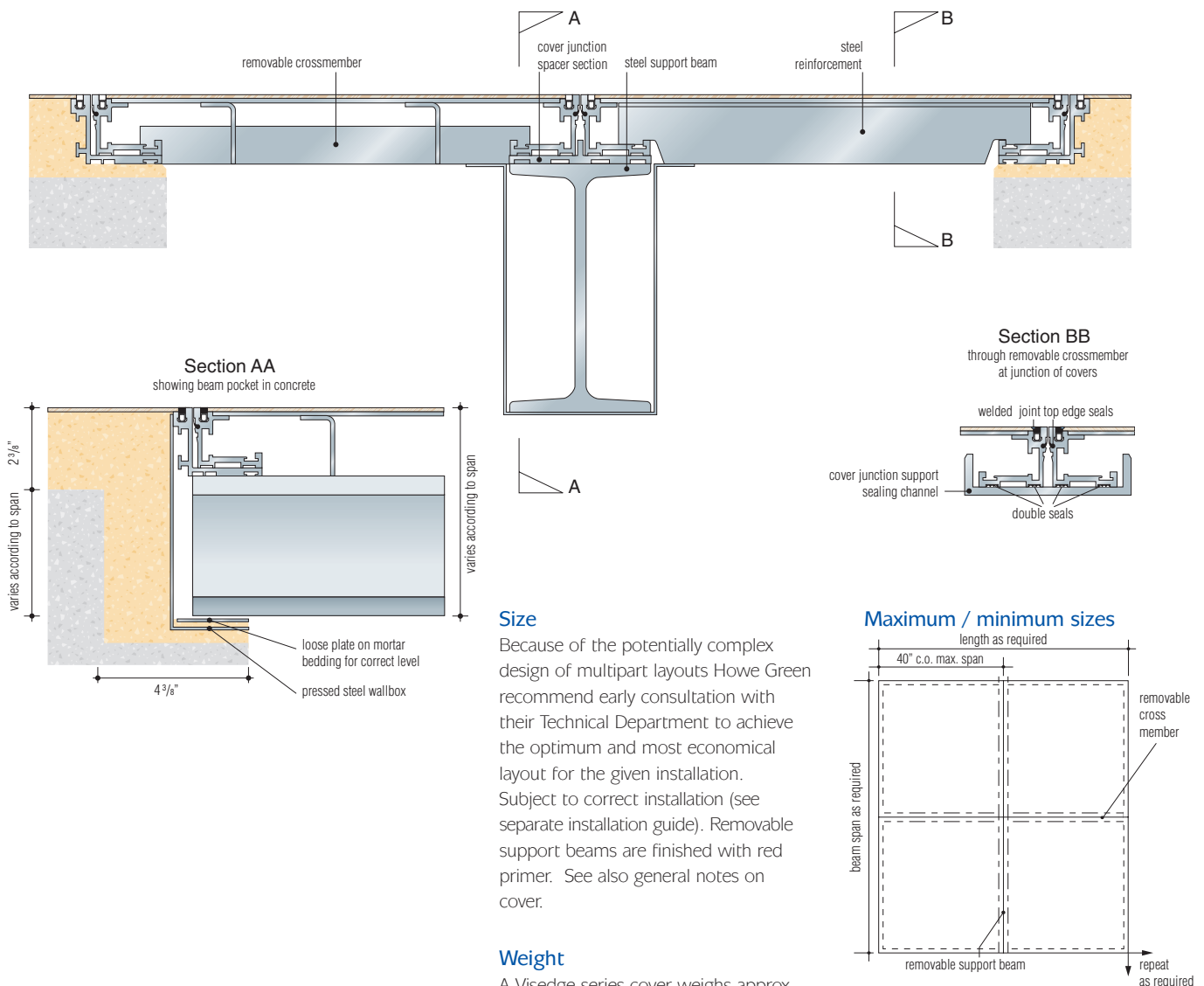
Cross section showing removable support beam and cross members (Scale 1:2)
